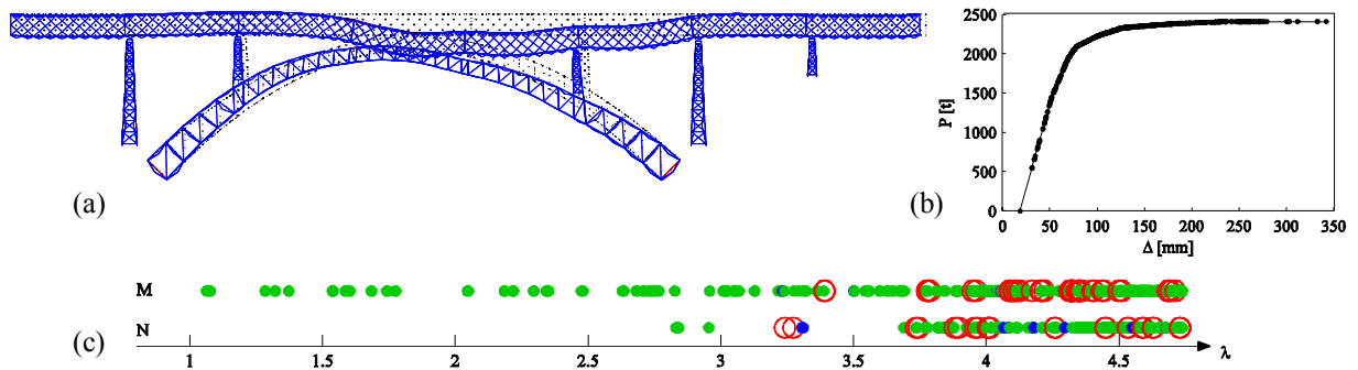
Fig. 4 Elastoplastic analysis of try-out Test I
