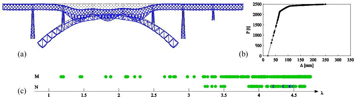
Fig. 5 Elastoplastic analysis of try-out Test II
