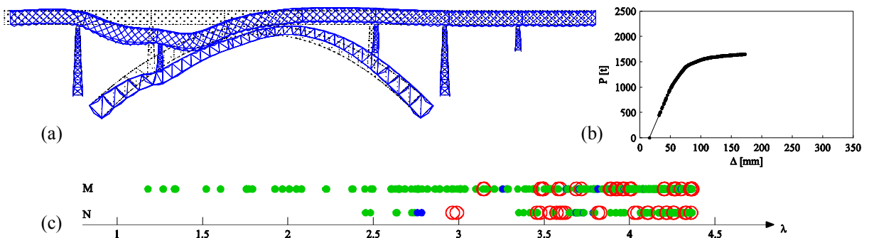
Fig. 7 Elastoplastic analysis of try-out Test IV
