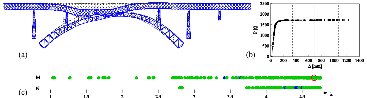
Fig. 6 Elastoplastic analysis of try-out Test III
