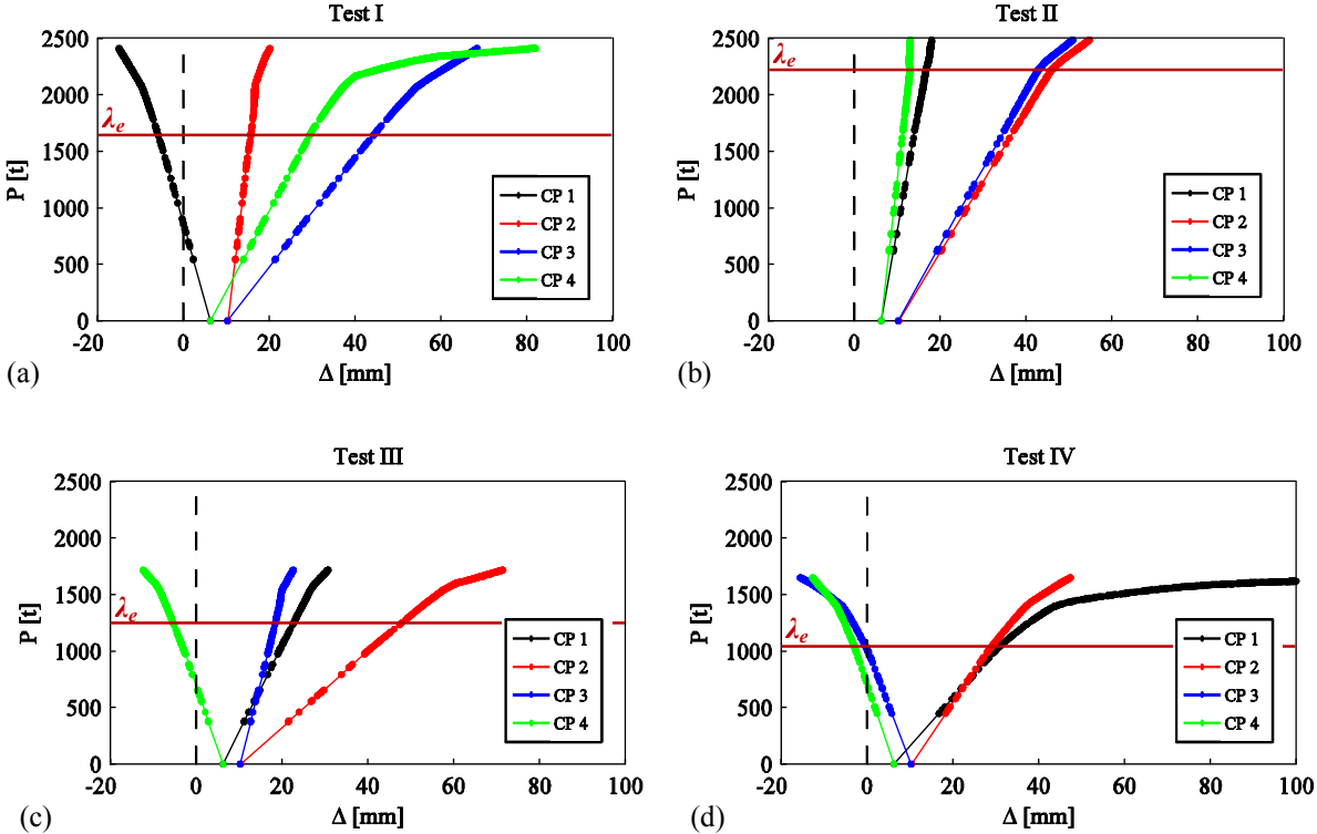
Fig. 8 Characteristic P-Δ curves at Control Points 1-4 (Fig. 3)
